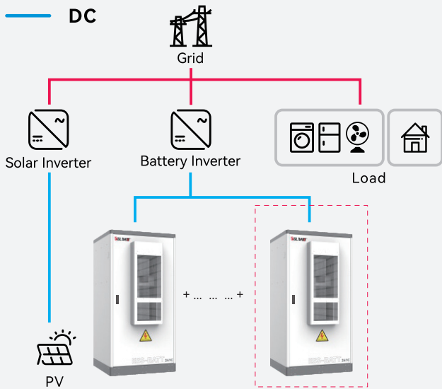
AC Coupled
